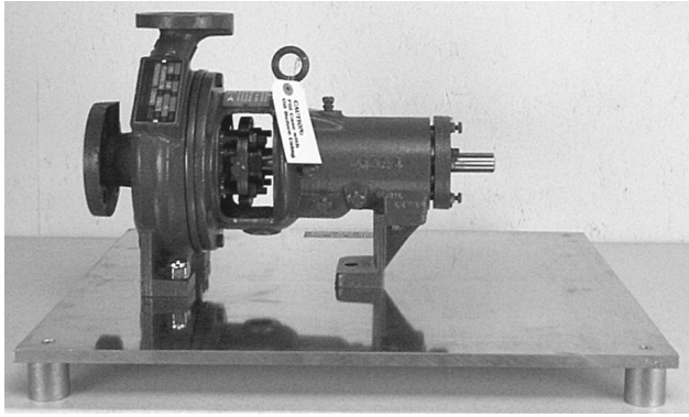
Model 3005 Pump Maintenance Trainer
