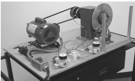
Model 3007-P Pneumatic Clutch and Brake
