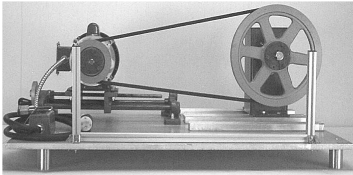
Model 3001 Belt Drive Trainer
