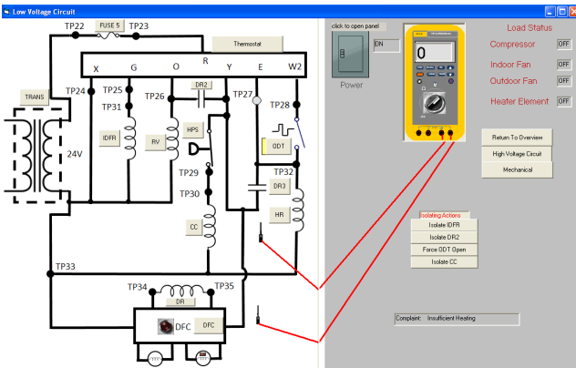
Low Voltage Electrical System
