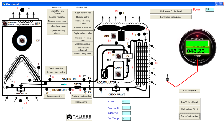
Mechanical System
