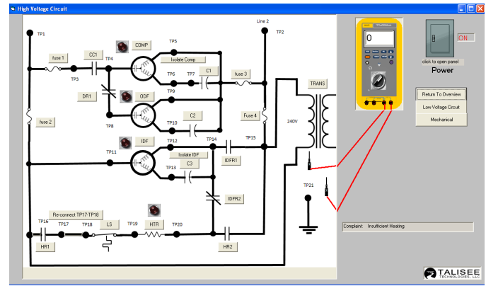
High Voltage Electrical System
